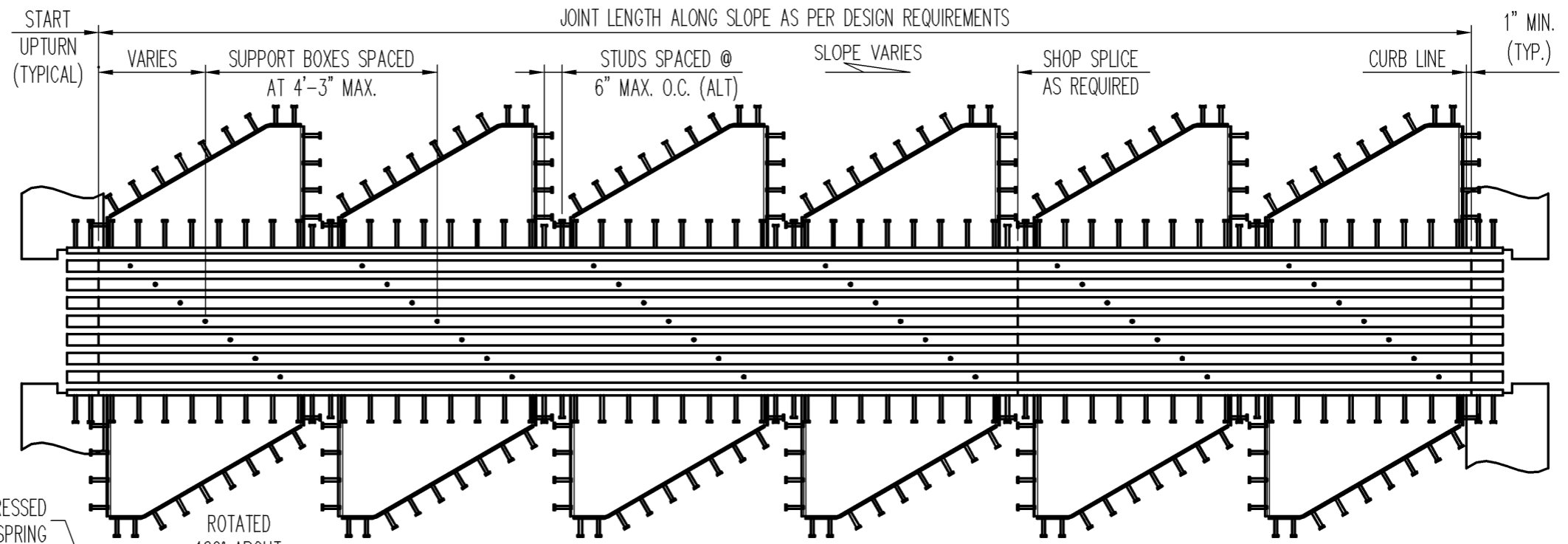
TYPICAL 'D-640' PLAN VIEW
