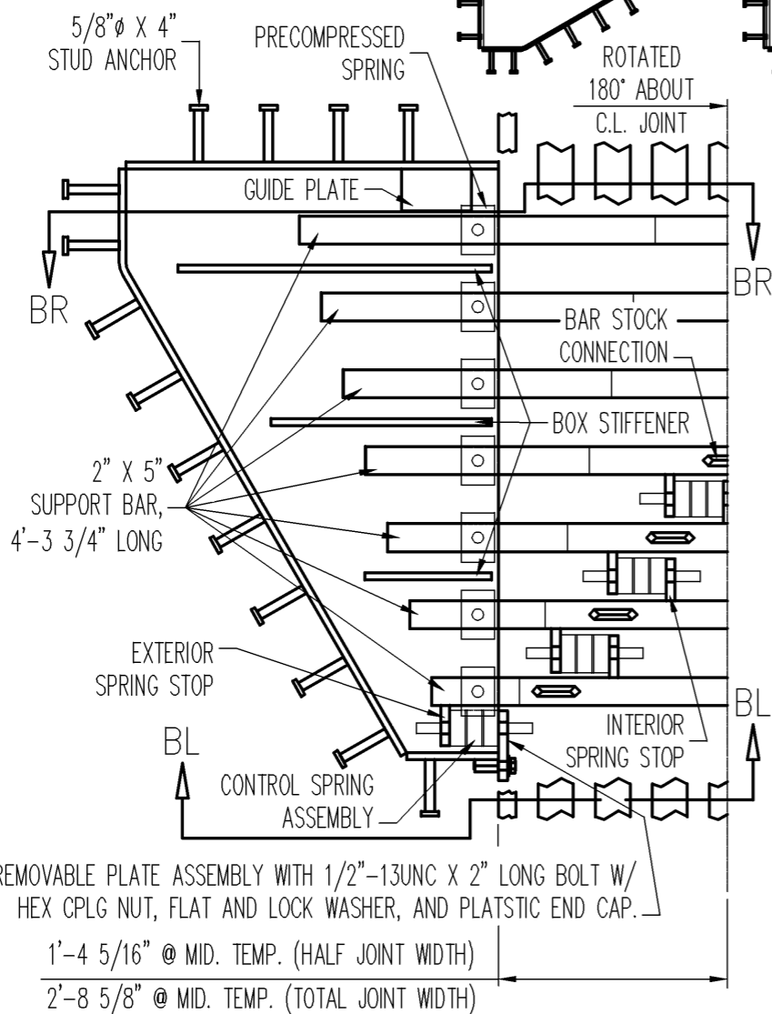
DETAIL "A" - PLAN VIEW OF 'D-640' EXPANSION JOINT @ SUPPORT BOX
