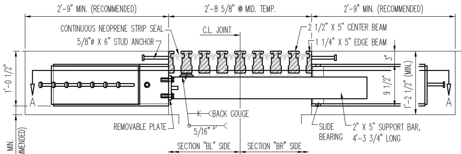
SECTION "B" - TYPICAL SECTION THROUGH 'D-640' EXPANSION JOINT @ SUPPORT BOX
