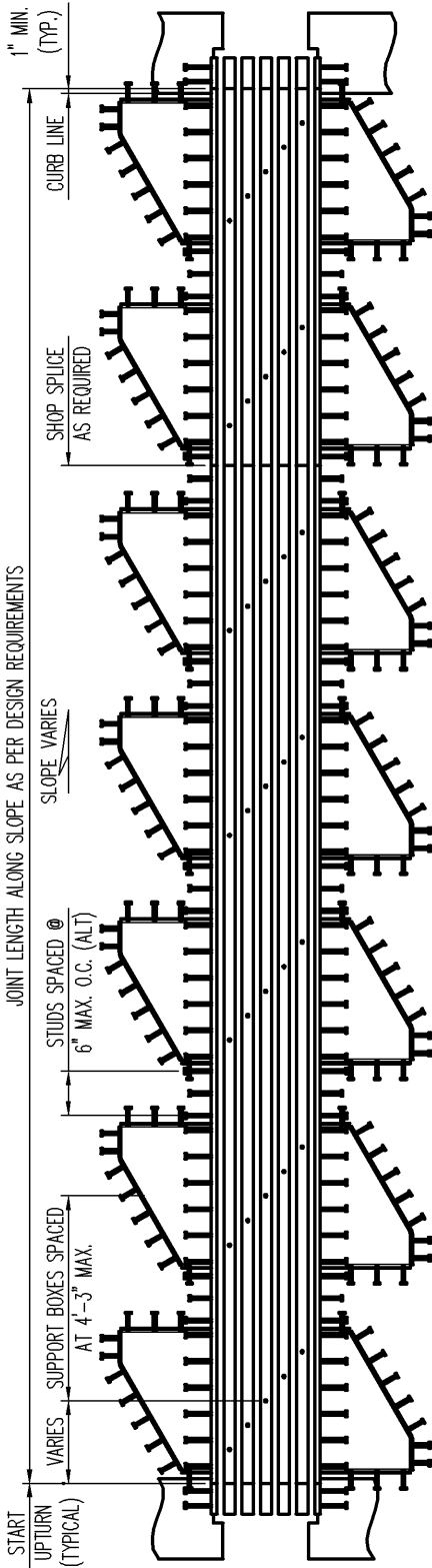
TYPICAL 'D-480' PLAN VIEW
