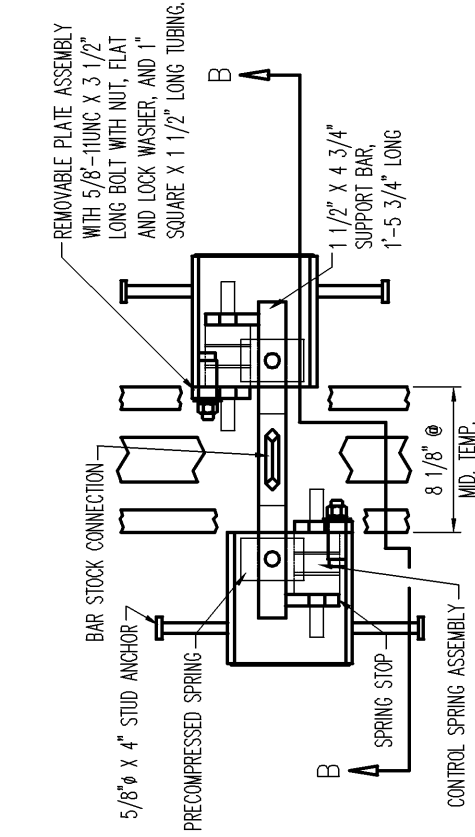
DETAIL "A" - PLAN VIEW OF 'D-160' EXPANSION JOINT @ SUPPORT BOX
