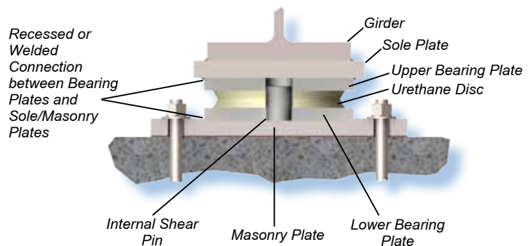
4-Plate Design
